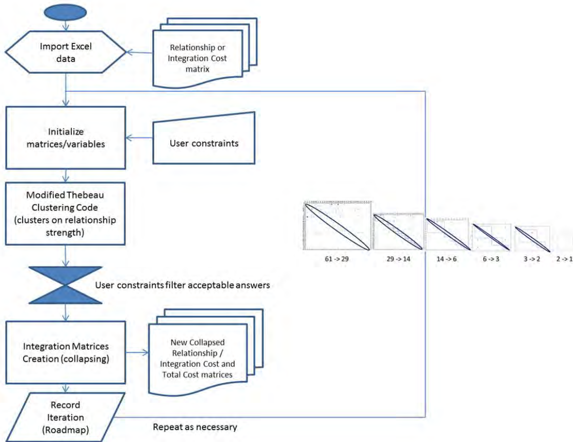
Figure 9. Collapsing DSM Algorithm Flowchart
