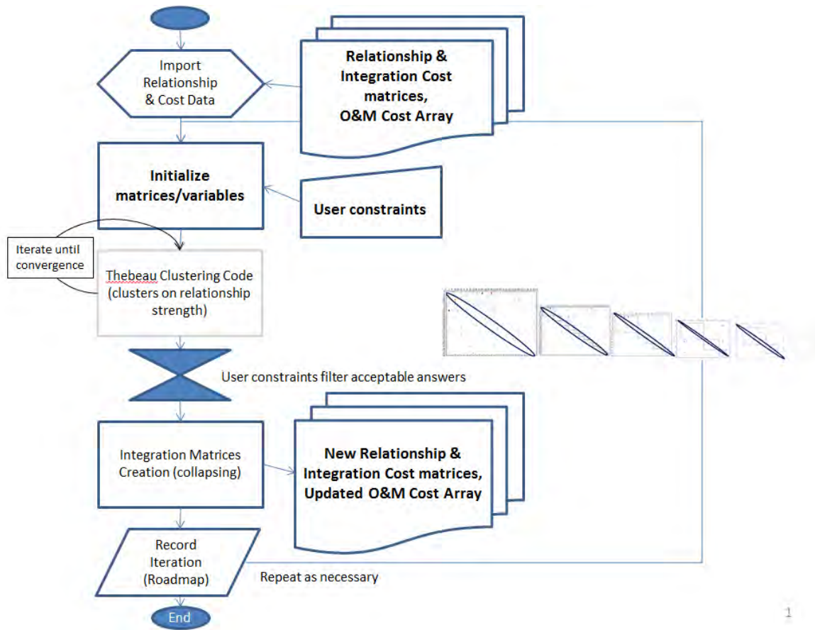
Figure 12. C-DSM Algorithmic Flowchart
